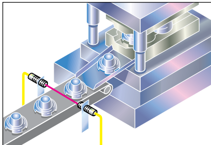
Diffuse photoelectric sensors verify parts count as parts move on conveyor.
