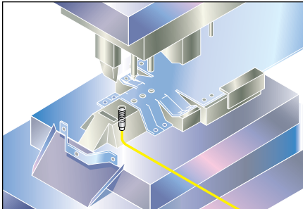
Inductive proximity sensor indicates correct hole positioning prior to each stamping hit.
