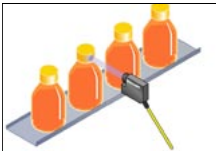
UV photoelectric sensor reads invisible tracer on medicine bottle cap to verify contents.
