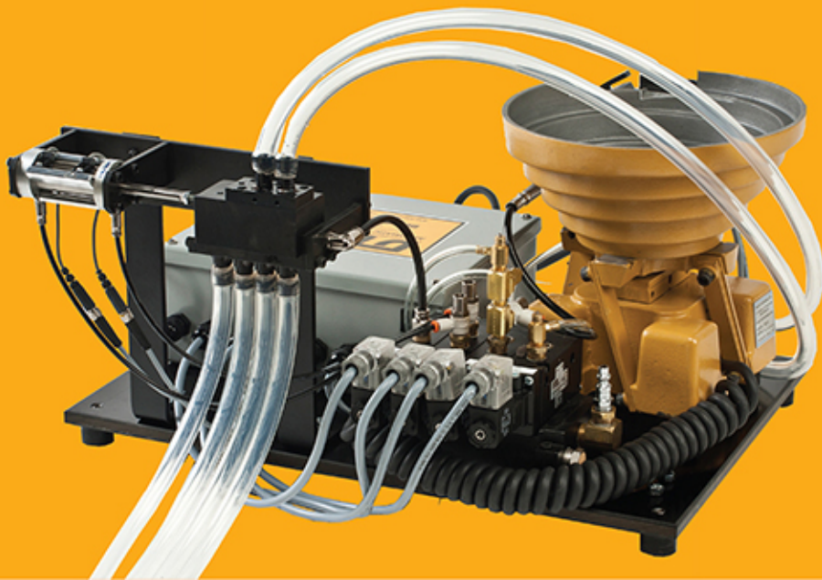
▲ Auxiliary supply hopper
