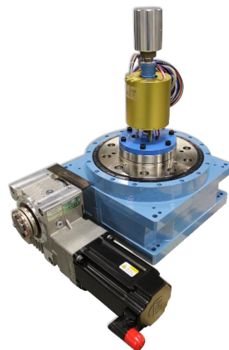
RT160 with Slip Ring and Rotary Air Union
