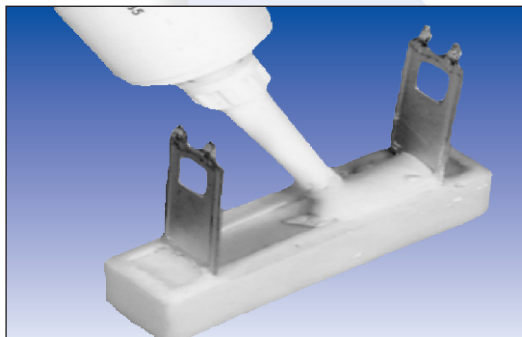
Applying 919 to a Hi-Power Resistor
